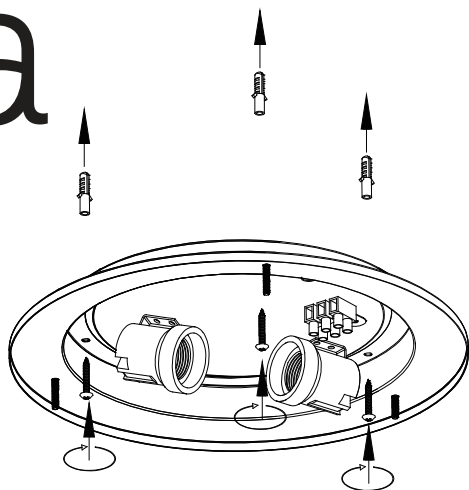
1. Fix the light body to wall or ceiling
