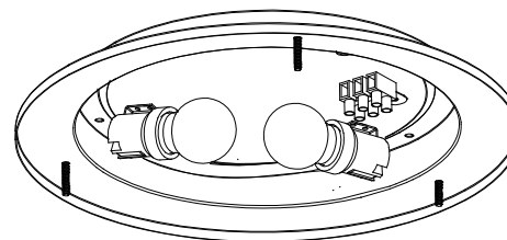
3. Install the light source
