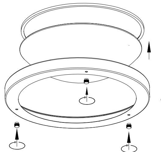
4. Fix the glass cover and the metal ring
